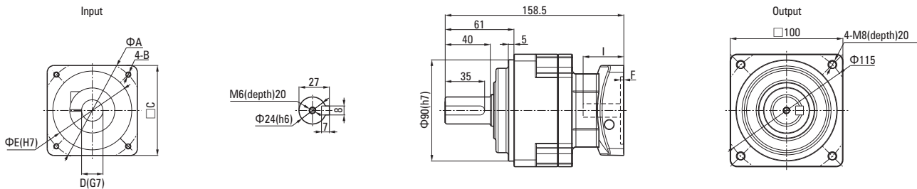
● Detailed Flange Dimensions Table
