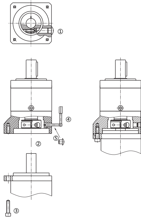
● HYE/F/WE/WF/S Series Schematic Diagram
